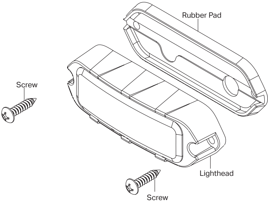
T3 Surface Mount
